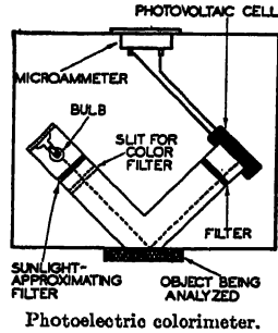
Photoelectric colorimeter.
